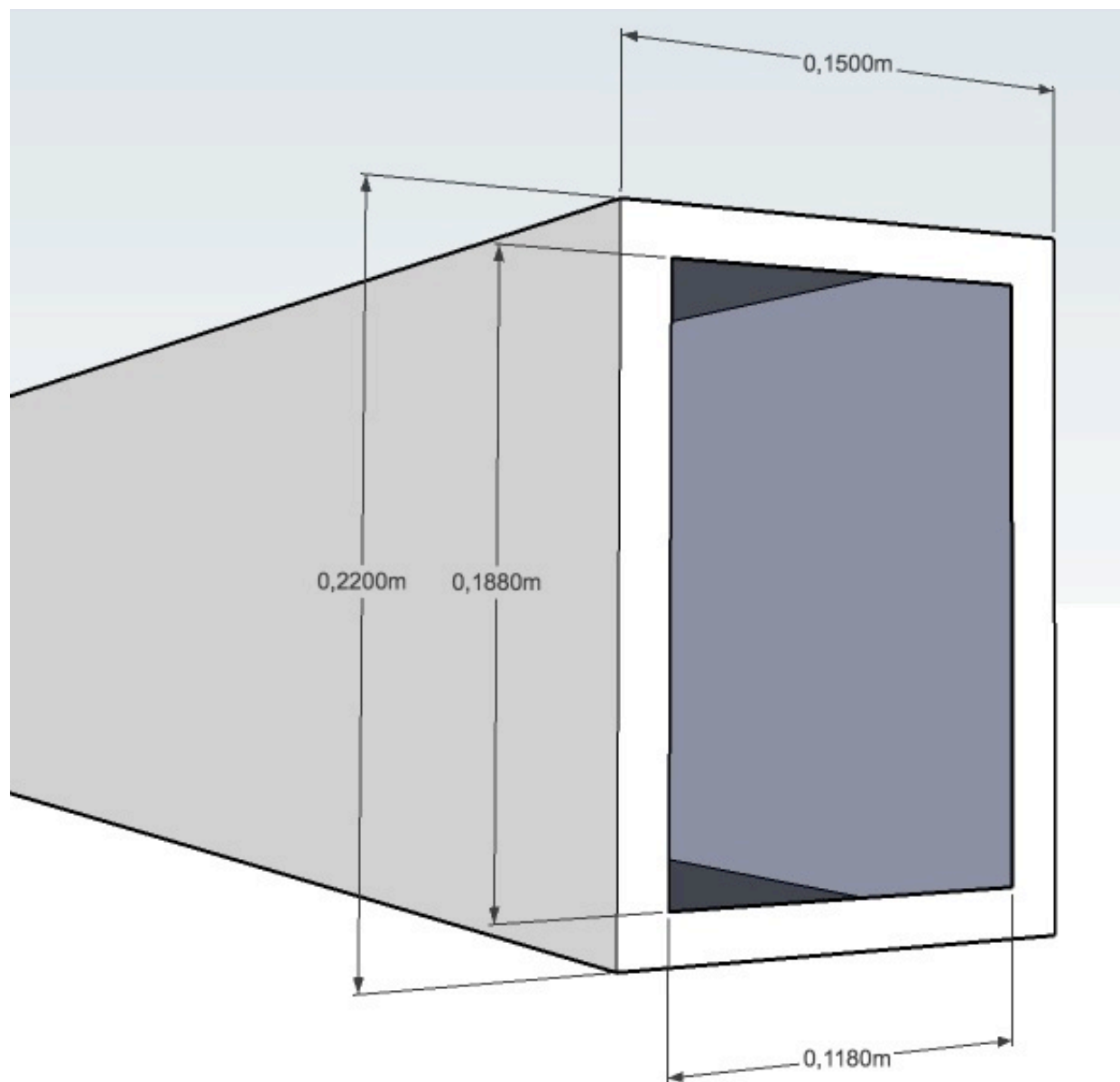
Fig 16: Piece 5 - connection to 6 and 1A
