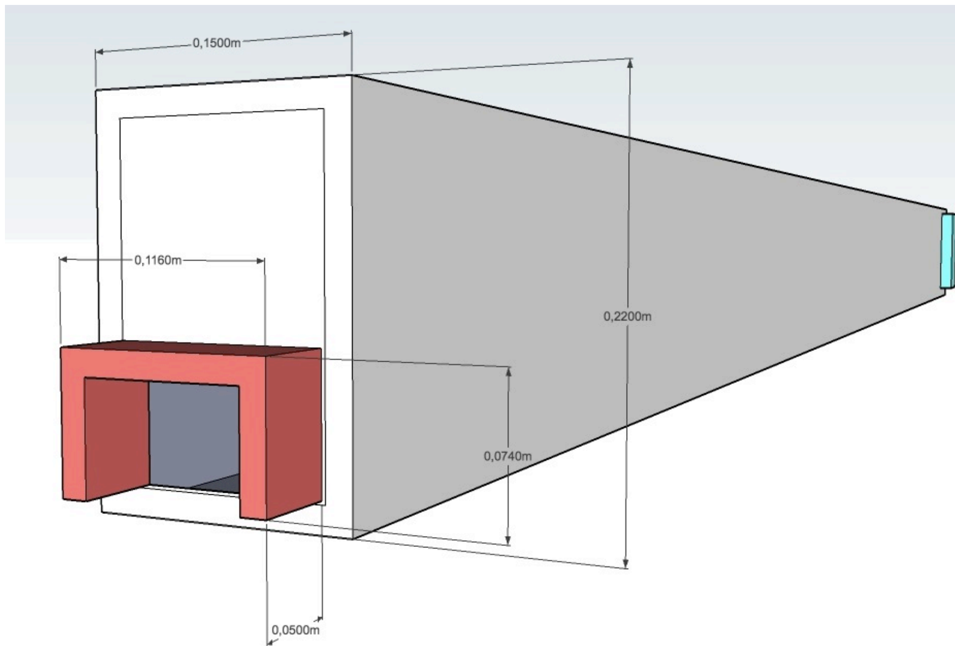
Fig. 22: Piece 1A - connection to door
